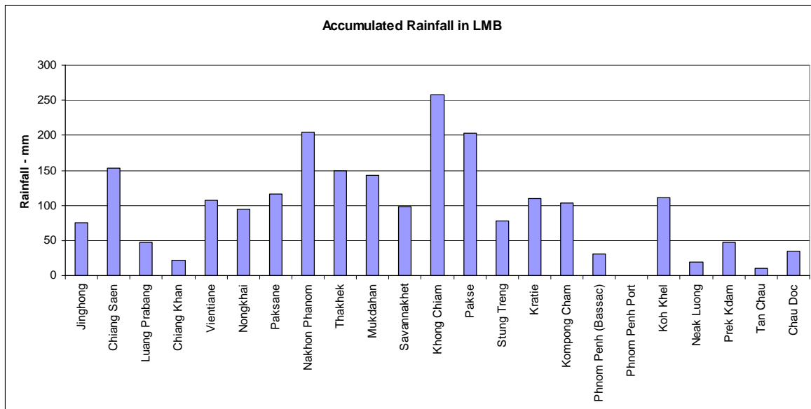
Figure 1: Accumulated Rainfall Distribution over the LMB from 10 th – 17 th July 2017
