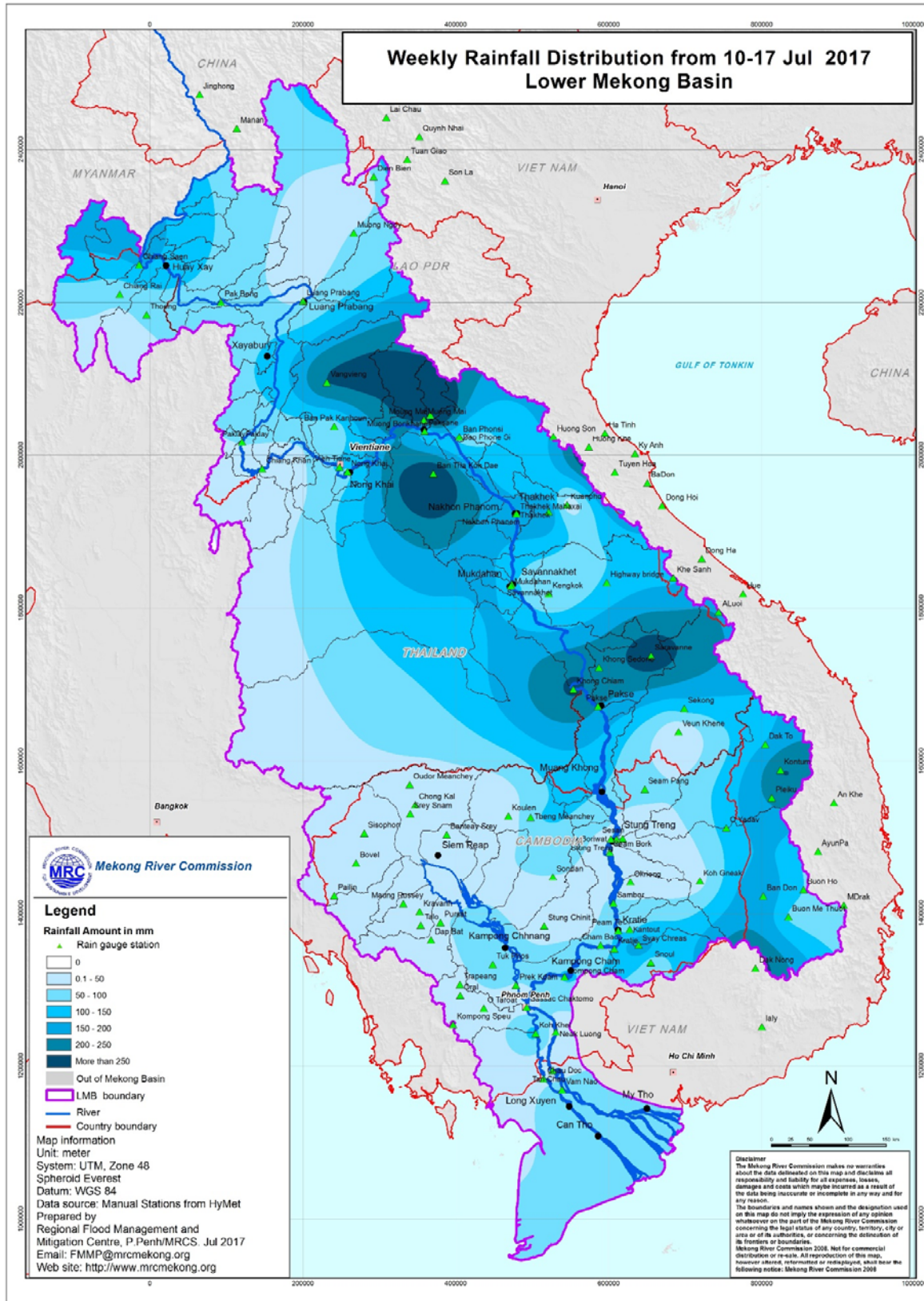
Figure 2: Weekly Rainfall Distribution over the LMB from 10 th – 17 th July 2017
