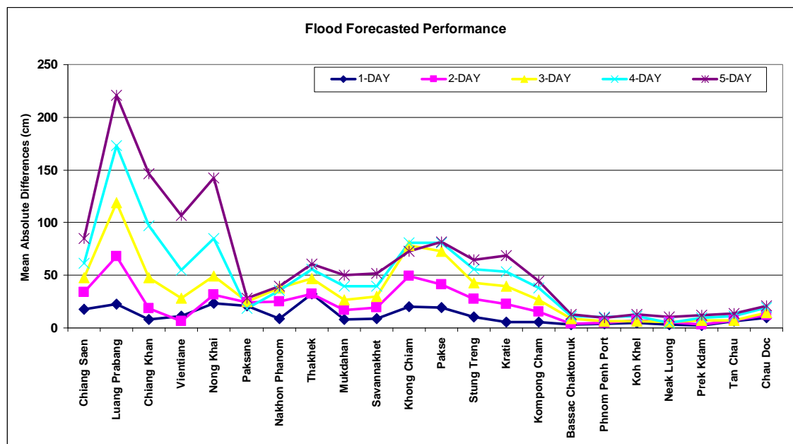
Figure B1: Average flood forecast accuracy along the Mekong mainstream (from 26 th June – 03 rd July 2017)
